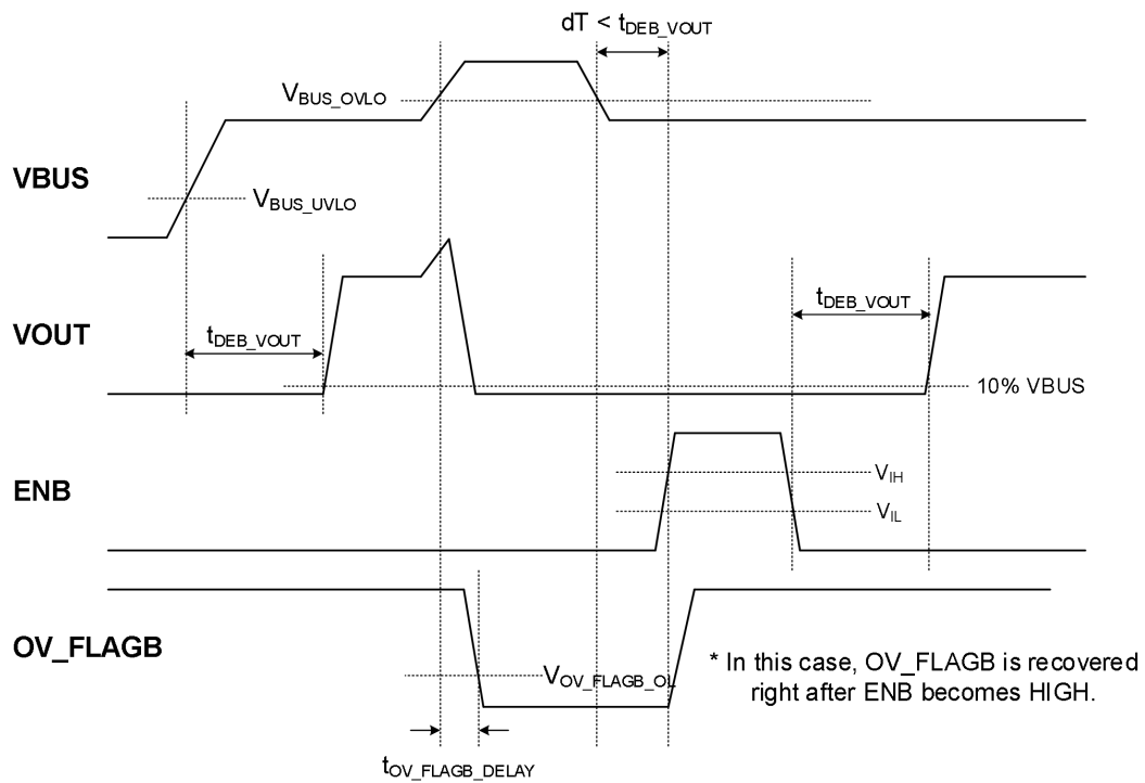
Figure4. VBUS OVLO Operation (ENB=High)
