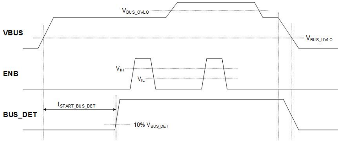
Figure6. VBUS_DET Operation
