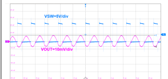
Figure22. Output Ripple
