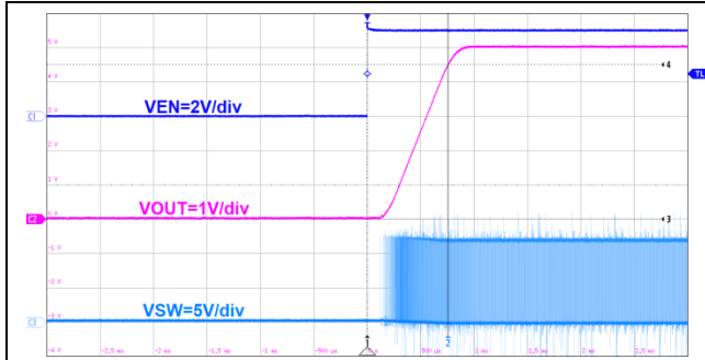
Figure67. Start-up by EN
