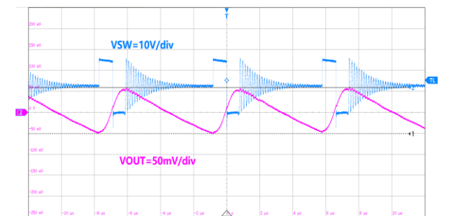
50us/div V_{OUT}=12.0V I_{OUT}=0.25A V_{IN}=24.0V Figure30. Output Ripple
