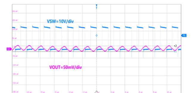
50us/div V_{OUT}=12.0V I_{OUT}=3.0A V_{IN}=24.0V Figure32. Output Ripple
