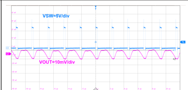
Figure20. Output Ripple
