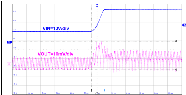
Figure59. Line Transient
