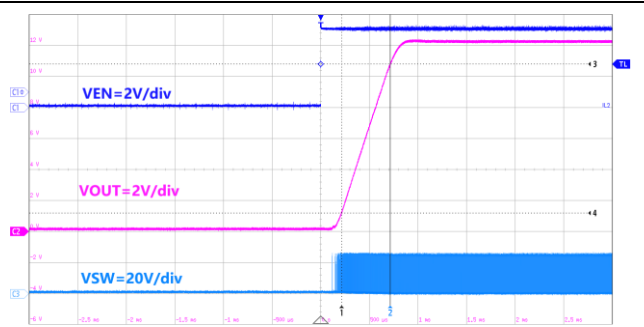
Figure68. Start-up by EN
