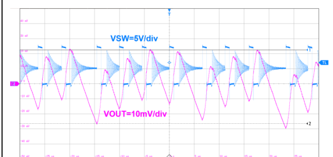
Figure24. Output Ripple
