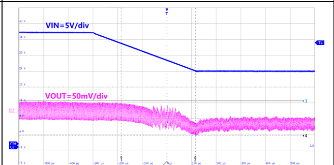
Figure62. Line Transient
