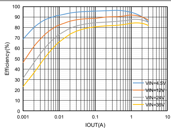
Figure6. Efficiency , V_{OUT}=3.3V
