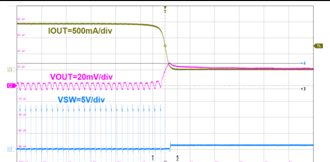
10us/div V_{OUT}=1.0V I_{OUT} = 1.5A to 0A Figure34. Load Transient
