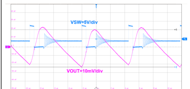
Figure20. Output Ripple
