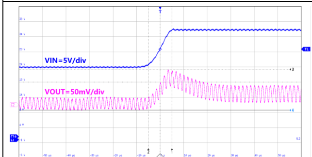
Figure61. Line Transient
