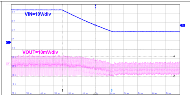
Figure60. Line Transient
