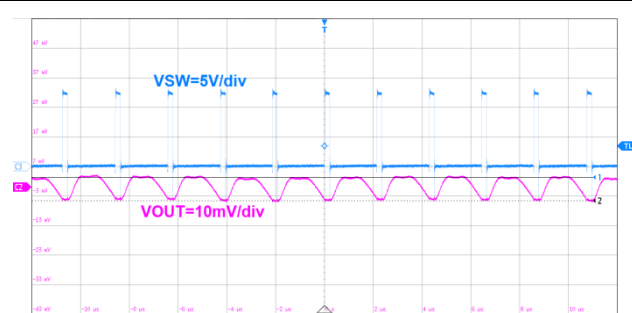
Figure19. Output Ripple
