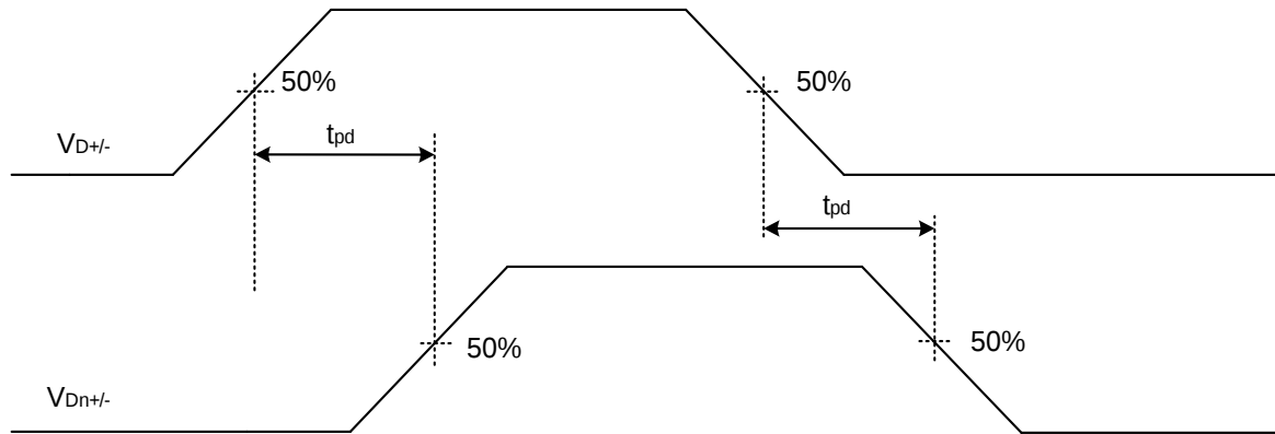
Figure 3. Propagation Delay
