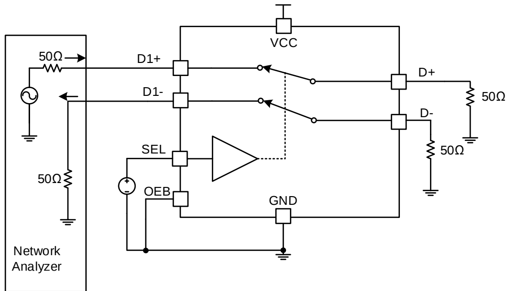
Figure 7. Crosstalk
