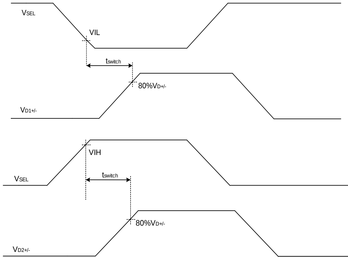
Figure 1. Switching Time Between Channels
