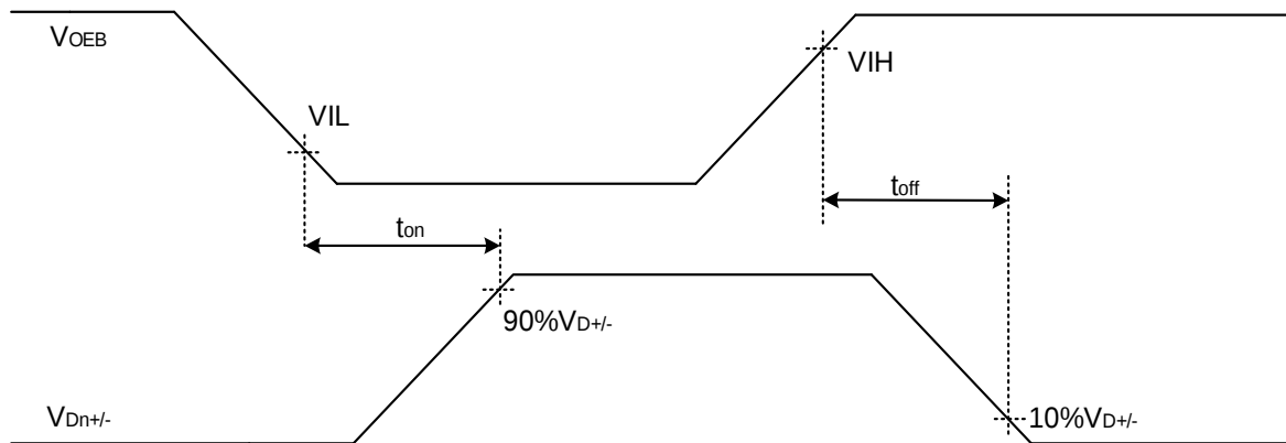
Figure 2. Device Turn On and Off Time
