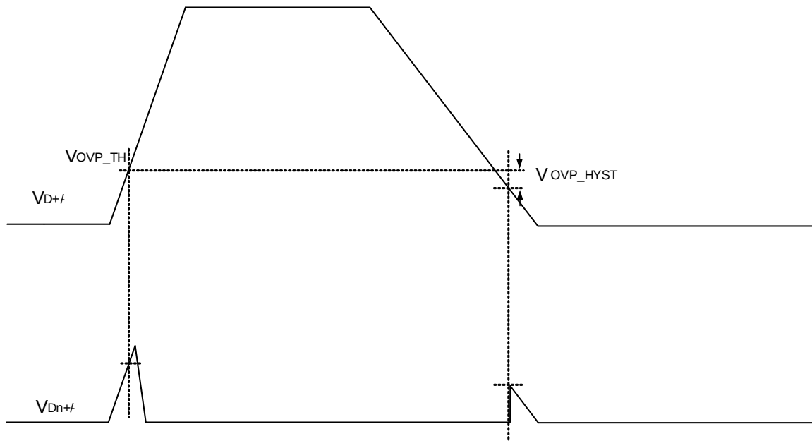
Figure 4. OVP Protection
