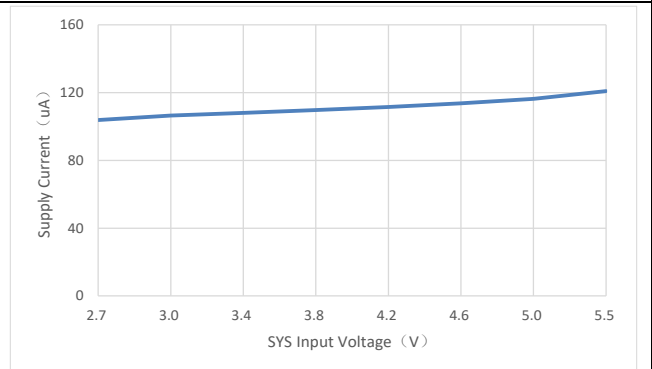
SYS Supply Current vs. SYS Input Voltage
