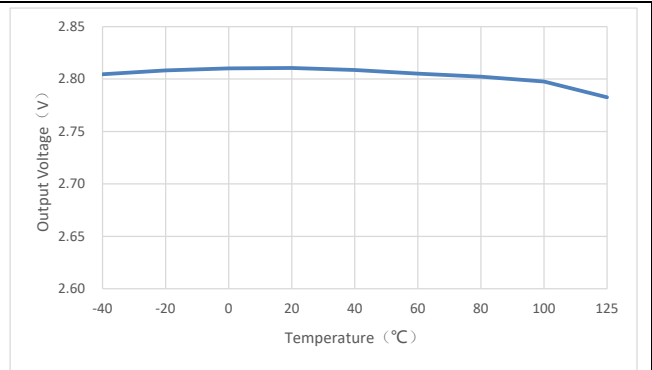
LDO3/4/5/6/7 Output Voltage vs. Temperature
