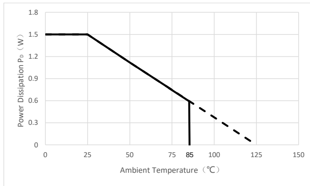
Power Dissipation
