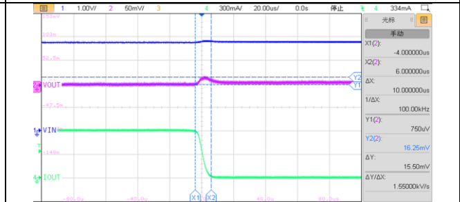
LDO3/4/5/6/7 Load Transient ( V_{IN3\sim 7}=3.8V , I_{OUT}=0.6A to 1mA )
