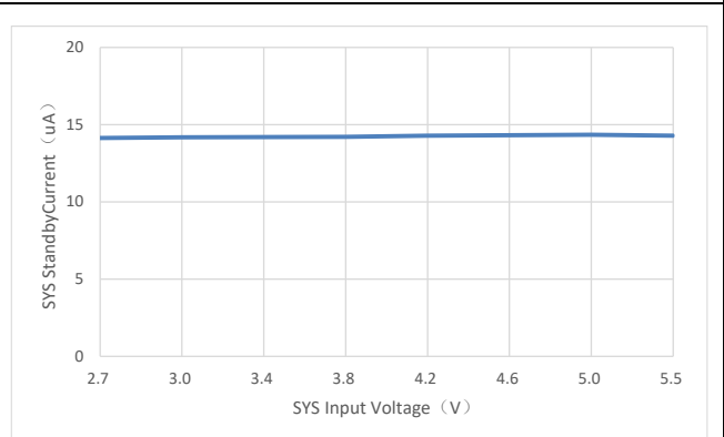
SYS Standby Current vs. SYS Input Voltage
