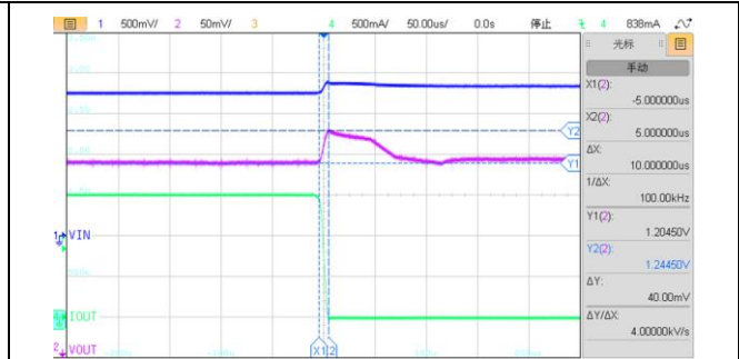
LDO1/2 Load Transient ( V_{IN12}=1.7V , I_{OUT}=1.5A to 1mA )
