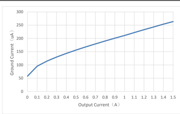
LDO1/2 Ground Current vs. Output Current
