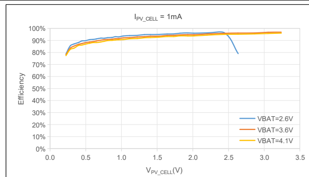
Figure 8. BOOST conversion efficiency ( I_{\text{PV\_CELL}}=1\text{mA} )
