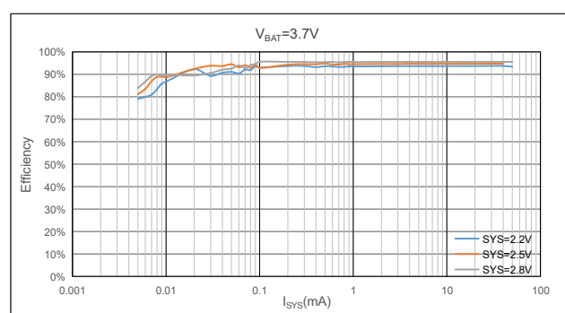
Figure 10. BUCK conversion efficiency ( V_{\text{BAT}}=3.7\text{V} )
