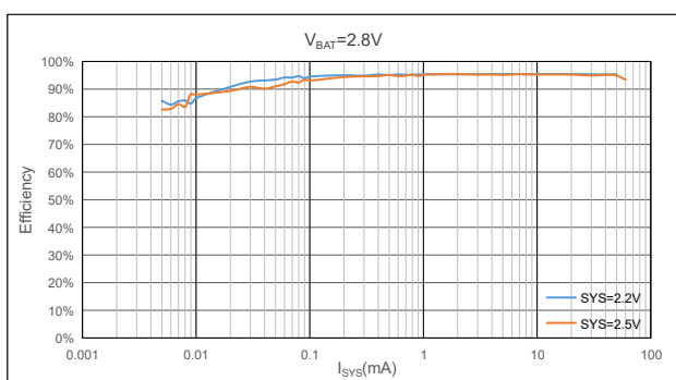
Figure 9. BUCK conversion efficiency ( V_{\text{BAT}}=2.8\text{V} )
