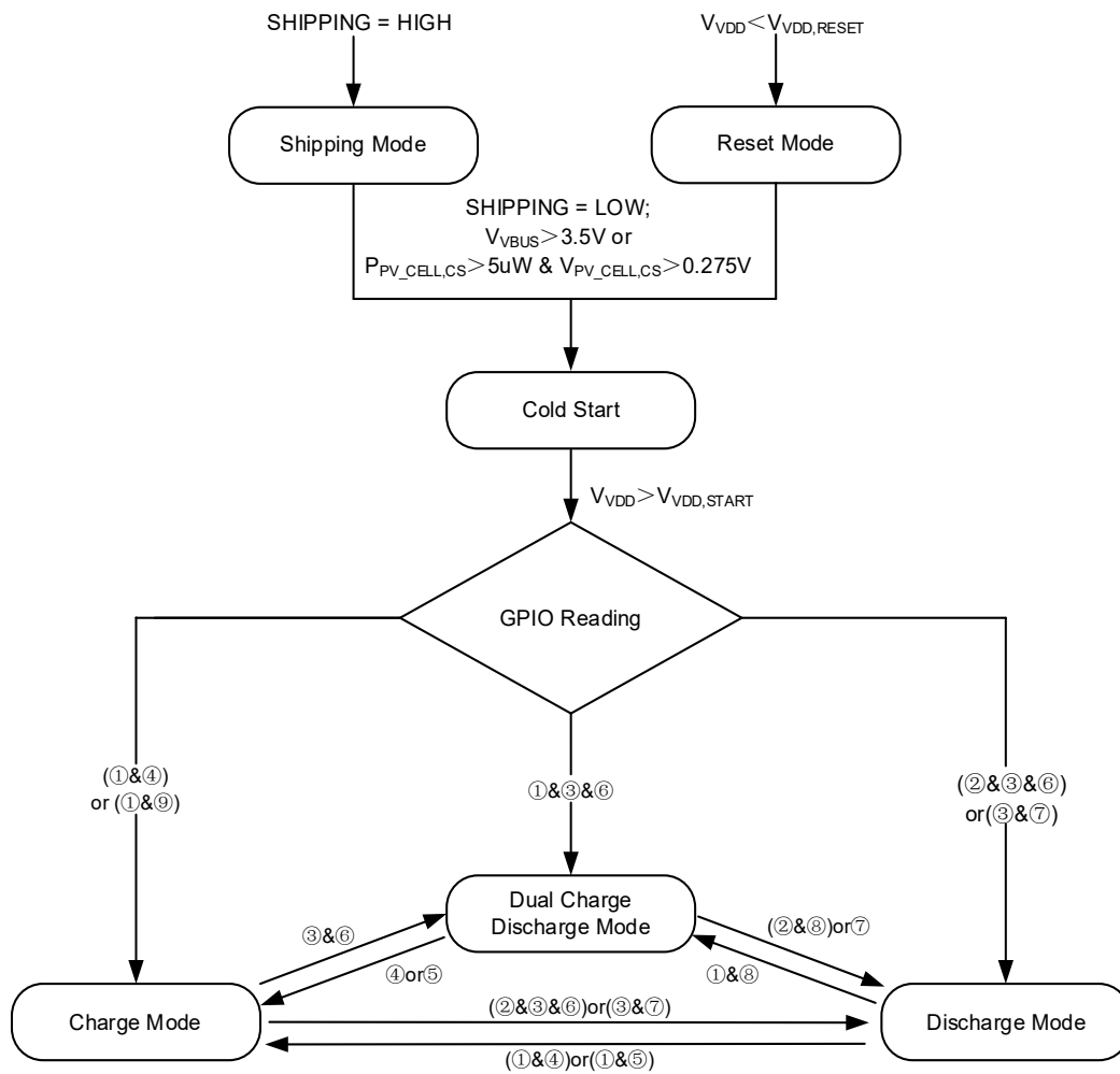
Figure 4. State Machine
