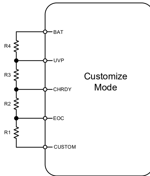
Figure 5. Custom configuration resistors
