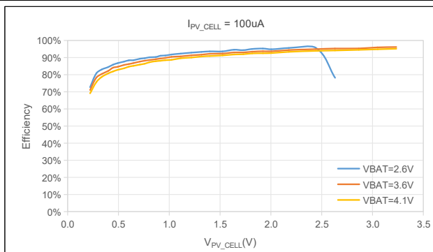
Figure 7. BOOST conversion efficiency ( I_{\text{PV\_CELL}}=100\mu\text{A} )
