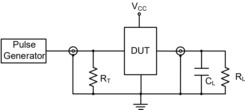
Figure 4. Test Circuit
