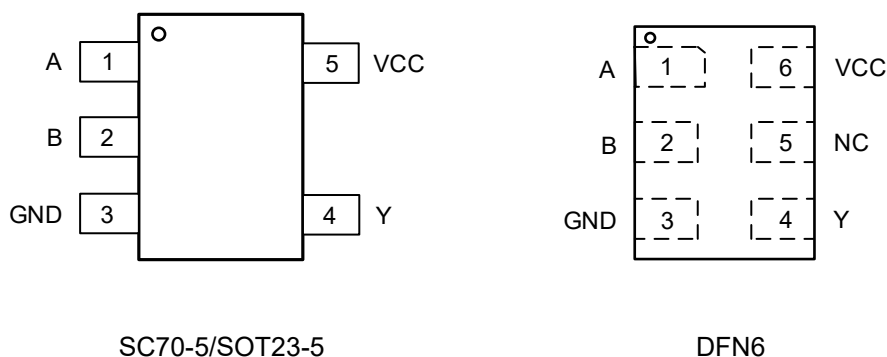
Top View Figure1. Pin Configuration
