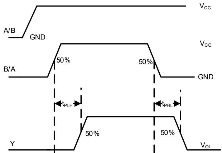
Figure 3. Switching Waveform
