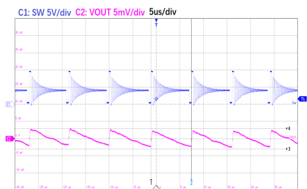
V_{OUT} = 9V I_{OUT} = 20mA Figure13. ET84501 Output Ripple
