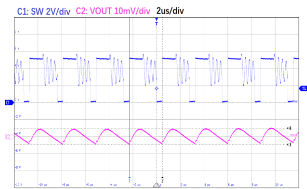
V_{OUT} = 5V I_{OUT} = 200mA Figure11. ET84501 Output Ripple
