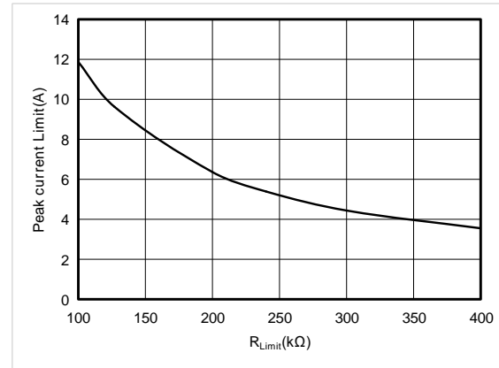
Figure9. ET84501 Switching Peak Current Limit Setting
