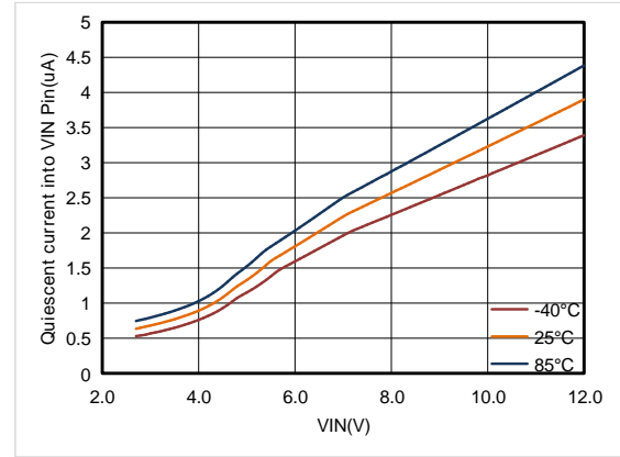
Figure3. ET84501 Quiescent current into VIN Pin
