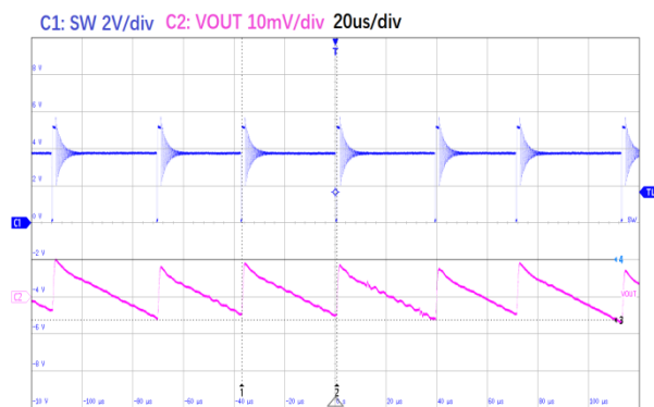
V_{OUT} = 5V I_{OUT} = 20mA Figure10. ET84501 Output Ripple
