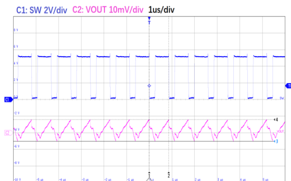
V_{OUT} = 5V I_{OUT} = 2A Figure12. ET84501 Output Ripple
