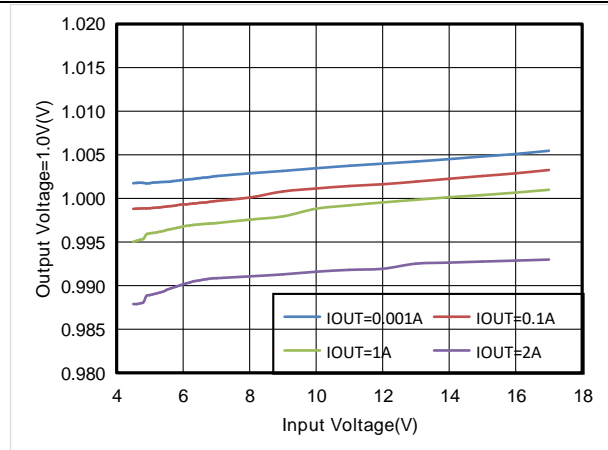
Figure14. ET8123 Line Regulation, V_{OUT}=1.0V
