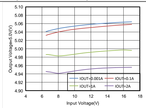
Figure16. ET8123 Line Regulation, V_{OUT}=5.0V
