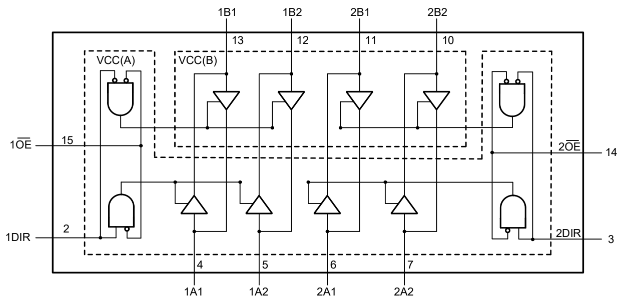
Figure2. Logic Symbol
