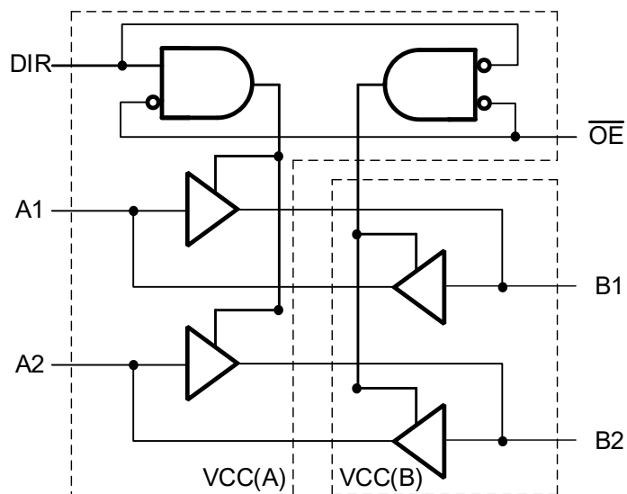
Figure3. Logic Diagram
