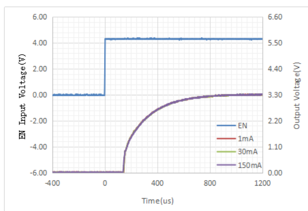
Turn On Speed VS EN Voltage
