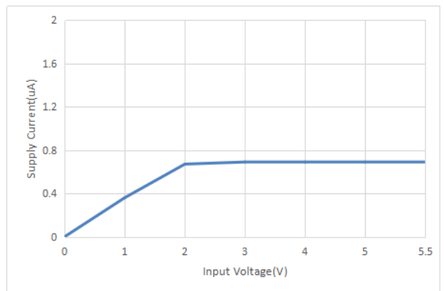
Supply Current VS Input Voltage
