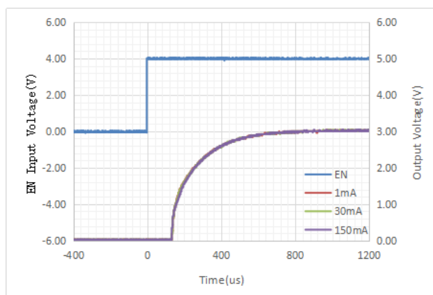
Turn On Speed VS EN Voltage
