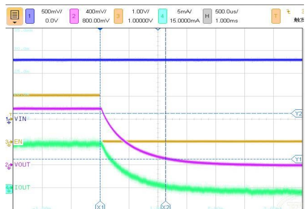
Turn Off VS EN Voltage ( I_{OUT}=10mA )
