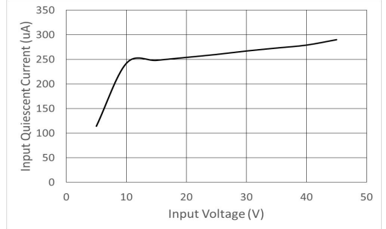
Input Quiescent Current vs. Input Voltage
